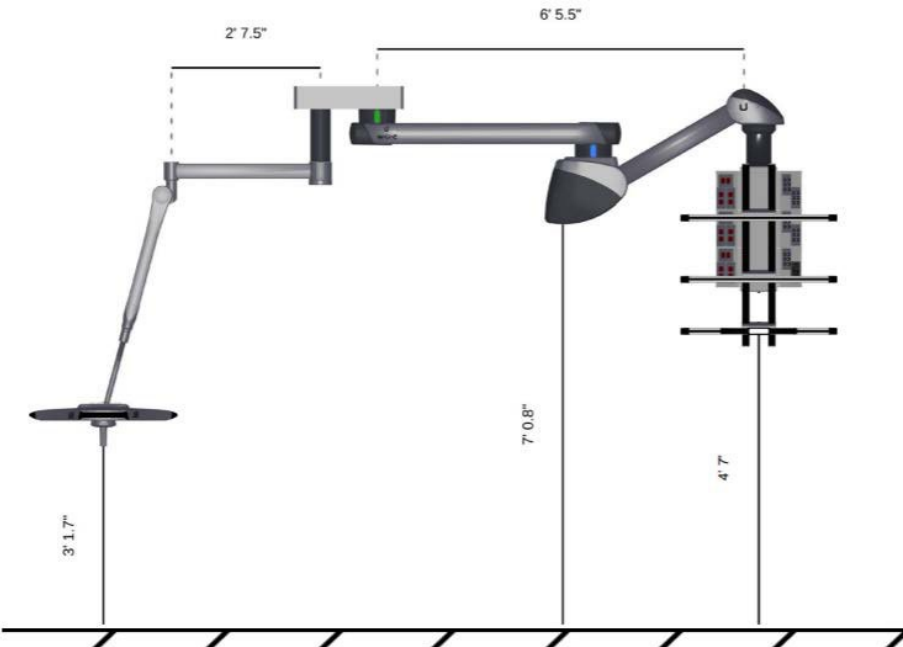
Configuration 1: Head Mounted Tandem Equipment Boom with Light
